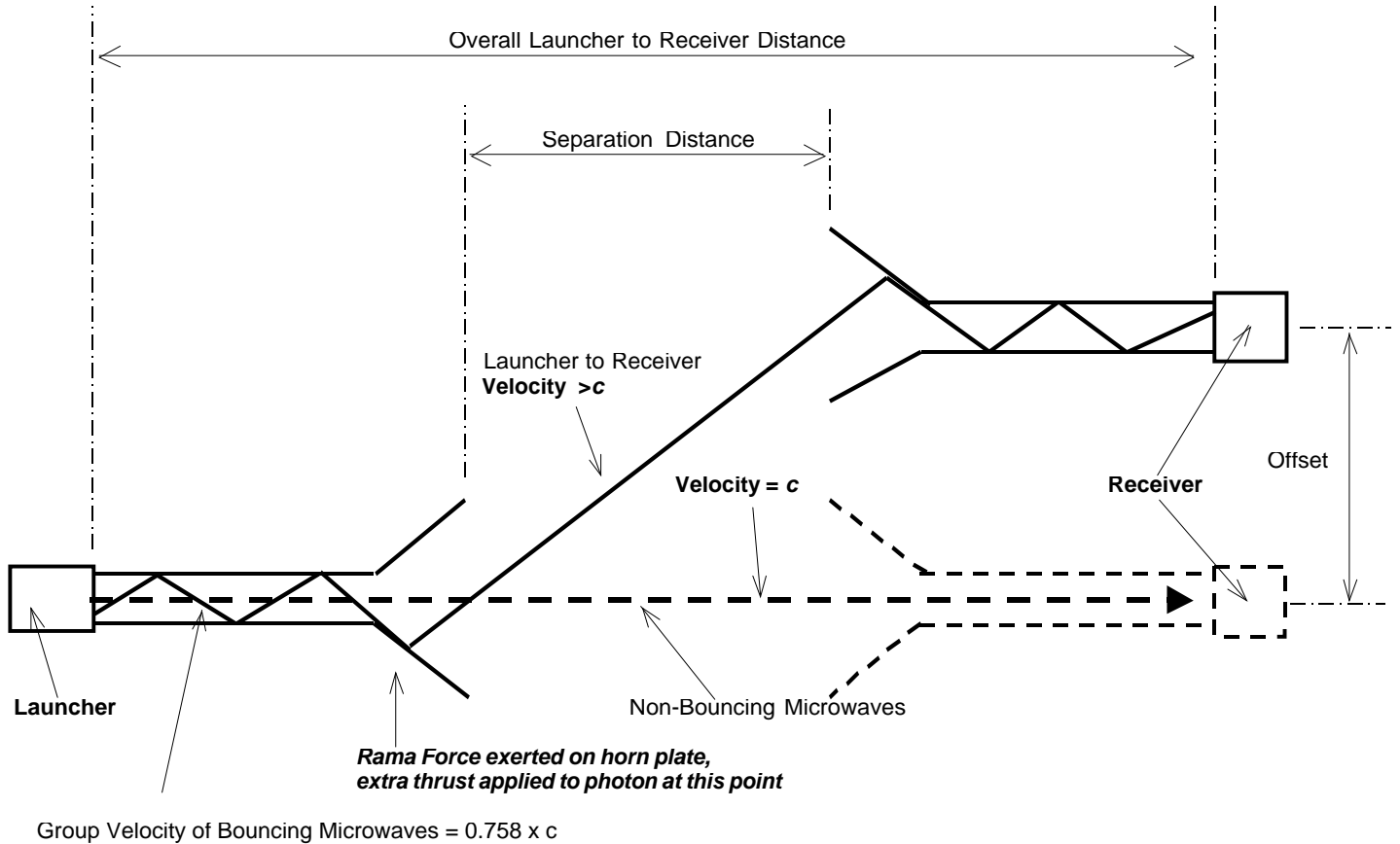
Figure 3. Ranfagni experiment (8) schematic showing Raman force effect on bouncing microwaves.
